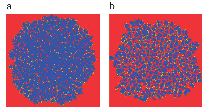
Fig. 2. Typical snapshots of the invasion of cooperators (blue) in a world of defectors (red) for (a) small cost-to-benefit ratio ( c/b = 0.02 ) and (b) for c/b closer to the extinction threshold ( c/b = 0.12 ). Along the interface separating cooperators and defectors, some individuals recently switched from defection to cooperation (green) or vice versa (yellow). (a) Cooperators expand as a single contiguous cluster with embedded specks of defectors, and a few isolated tiny cooperator formations along the invasion front. In this snapshot there is one large cluster of size 23187 accompanied by 14 single, isolated cooperators and the average weighted cluster shape is \gamma = 0.078 . The fraction of cooperators is f_c = 0.58 and q_{c|c} = 0.89 . (b) Cooperators form numerous small compact clusters. There are 143 clusters ranging from a single cooperator to a cluster of size 1987, with a weighted average size of 537 and shape \gamma = 0.356 . The fraction of cooperators is f_c = 0.37 and q_{c|c} = 0.76 . The snapshots are shown for an initial 15 \times 15 cluster on a 200^2 lattice and can be reproduced using the VirtualLabs (Hauert, 2006b).
