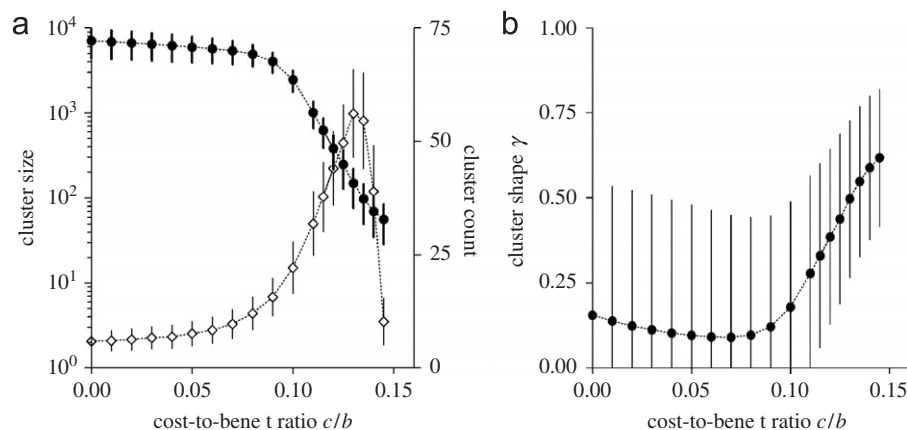
Fig. 3. Macroscopic features of the invasion of cooperators: (a) cluster size (●) and count (◇) as well as (b) cluster shape \gamma for increasing cost-to-benefit ratios c/b . (a) As suggested by the snapshots in Fig. 2, the cluster size decreases with c/b , while the number of clusters increases. For c/b < 0.1 , few sizeable clusters dominate the expansion, which means that the cluster size keeps increasing as invasion continues. In contrast, the big clusters break up and numerous small clusters are formed for c/b > 0.1 . (b) The same two distinct regimes are reflected in the mean cluster shape \gamma weighted by the cluster size. For c/b < 0.1 , \gamma is very low because of numerous embedded specks of defectors but displays a large variance due to their variable numbers. In contrast, compact clusters with convex shapes form for c/b > 0.1 such as to minimize interactions with defectors. For an initial cluster of 15 \times 15 cooperators, the cluster size, count and shape are determined when cooperators reach the boundary of a 115^2 lattice and averaged over 1000 runs. Cluster size and shape are weighted by the cluster size (see text). Vertical bars indicate the standard deviation (the standard error lies within the size of the symbols).
