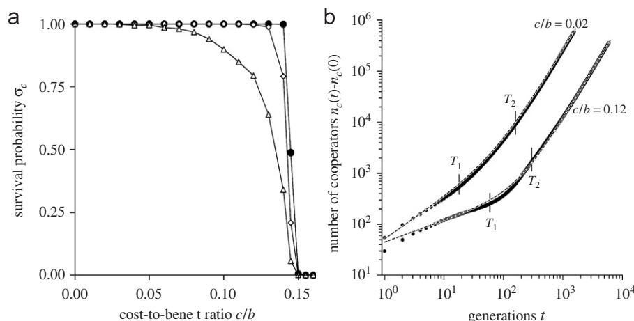
Fig. 1. Survival probability \sigma_C and growth characteristics of invading cooperators. (a) For initial cluster sizes of s \times s with s \geq 3 , the survival probability is close to 1 and essentially independent of s ( \Delta, s = 3 ; \diamond, s = 5 ; \bullet, s = 15 ) and the cost-to-benefit ratio c/b up to the extinction threshold \lambda \approx 0.15 , where cooperators can no longer survive irrespective of their initial abundance. \sigma_C is determined over 1000 runs on a 115 \times 115 lattice and cooperators are assumed to survive if they reached the boundary. (b) The growth of the number of cooperators n_c(t) displays two distinct regimes: a first phase of slow growth that corresponds to a local equilibration process of the initial cluster, followed by a second phase representing the expansion of cooperators. Both regimes follow a power function of the form n_c(t) = a_i t^{d_i} but with distinct growth exponents ( d_1 < 1 in the first phase and d_2 \approx 2 in the second phase; see Table 1). For the fits and the growth curve in panel (b), the initial number of cooperators n_c(0) was subtracted. The dashed line shows the superposition of the two fits n_c(t) = a_1 t^{d_1} + a_2 t^{d_2} . Vertical lines mark the end of the first ( T_1 ) and the beginning of the second growth phase ( T_2 ) as used for fitting the power function. The expansion process is shown for a 30 \times 30 cluster on a 1000^2 lattice ( n_c(0) = 900 ) averaged over 100 runs.
