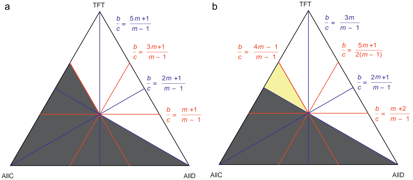
Fig. 3. Strategy abundance in the interaction between AIIc, AIID, and TFT in the probability simplex S_3 . Dark areas are inaccessible to the evolutionary dynamics. Red lines show thresholds where a strategy abundance crosses \frac{1}{3} , the thresholds are given in terms of b/c . Blue lines depict thresholds where two strategy abundances are identical. (a) For small mutation rates, the abundance of AIIc is never above \frac{1}{3} and it is never greater than the abundance of TFT. (b) For high mutation rates, the abundance of AIIc is above \frac{1}{3} in the yellow shaded area, but again it never exceeds the abundance of TFT. (For interpretation of the references to colors in this figure legend, the reader is referred to the web version of this article.)
